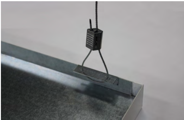
Mounting bracket showing indicative suspension equipment (suspension equipment supplied by others)
